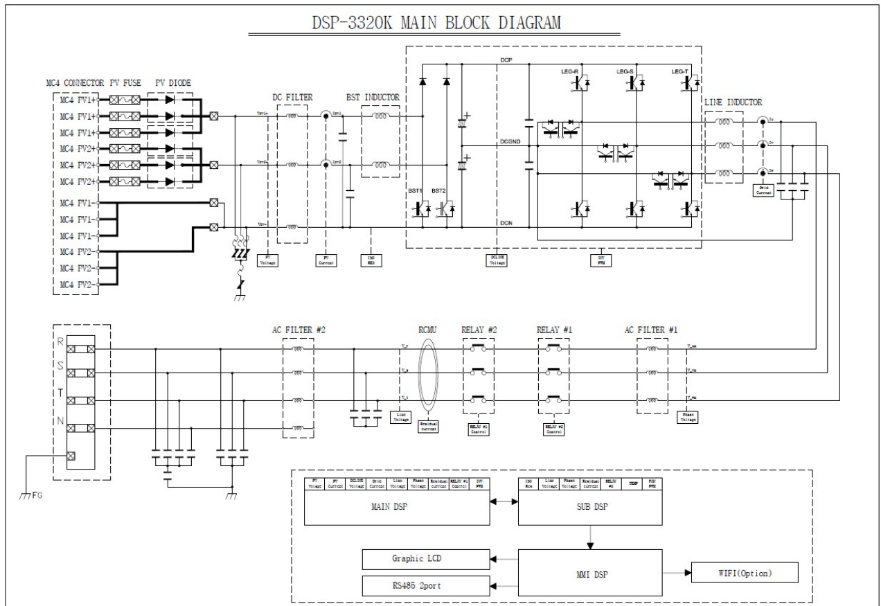
<DSP-3320K-OD Block Diagram>
